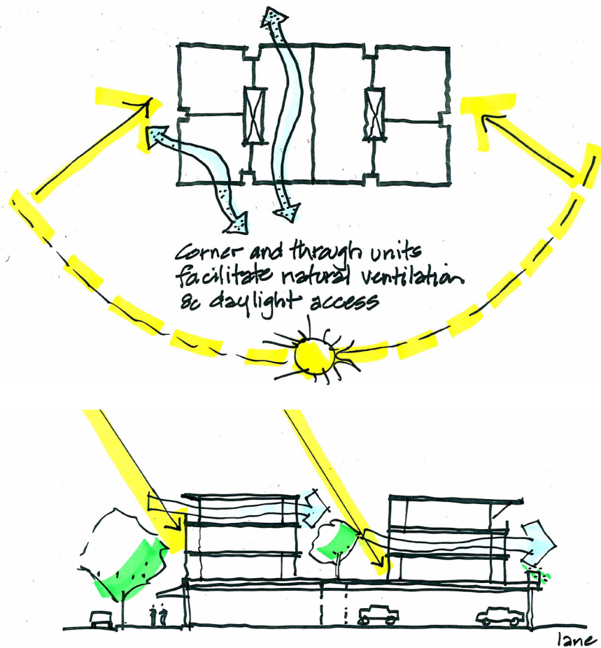
Dual-aspect homes enable enhanced access to daylight and natural ventilation.
