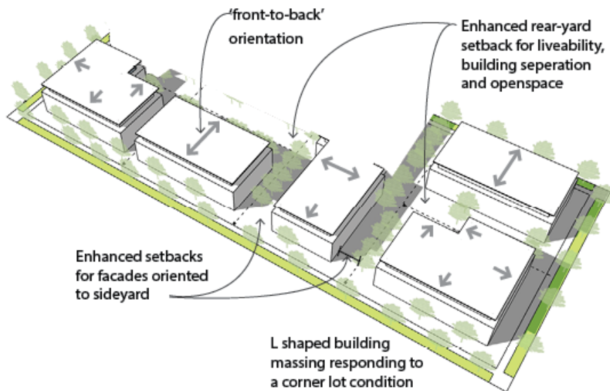
Perimeter block definition and livability is improved by enhanced setbacks for primary facades facing side yards and L-shaped massing on corner lots.
