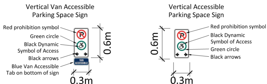
Figure 4: Accessible parking sign specifications
