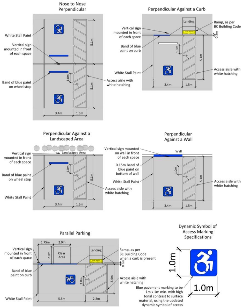
Figure 3: Minimum Van Accessible Parking Space dimensions
