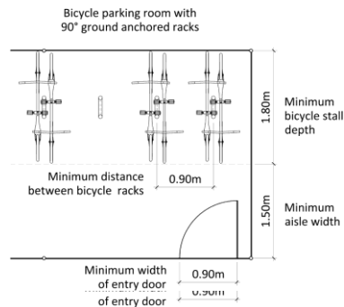
Example: Bicycle Parking Long-Term Configurations
