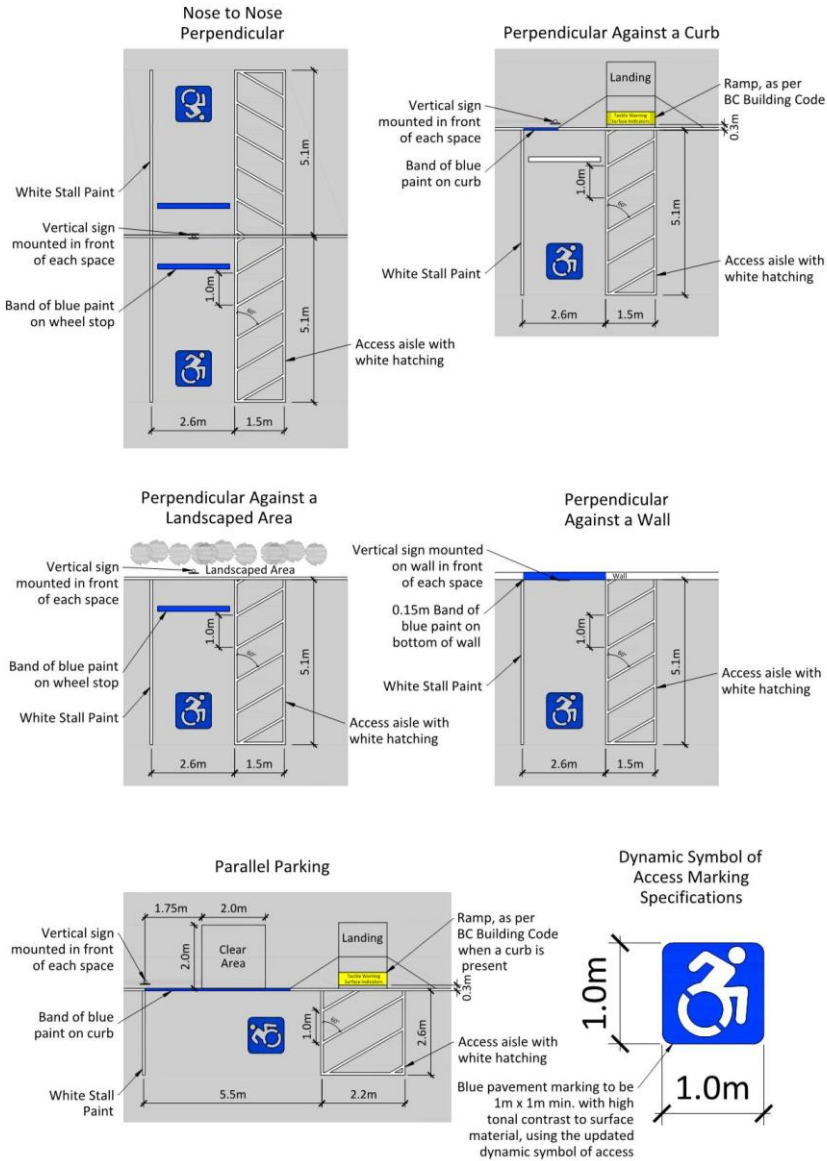
Figure 2: Minimum Accessible Parking Space dimensions
