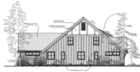
Side (E) Elevation Scale: 1:100
