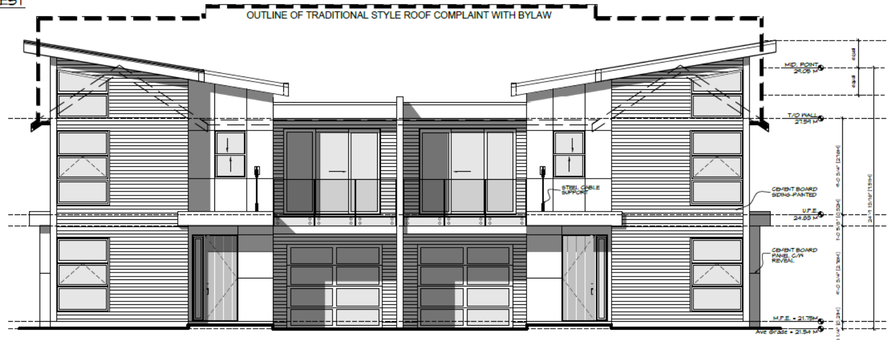
FRONT ELEVATION
