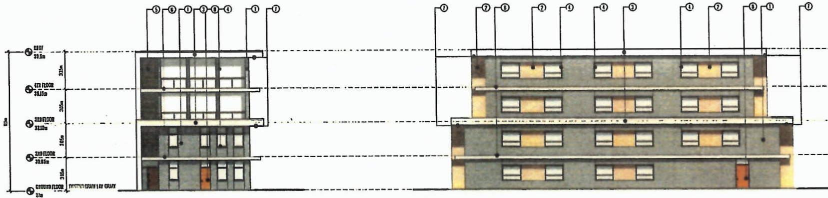
WEST ELEVATION
