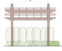
Wood Pergola - Front Elevation
