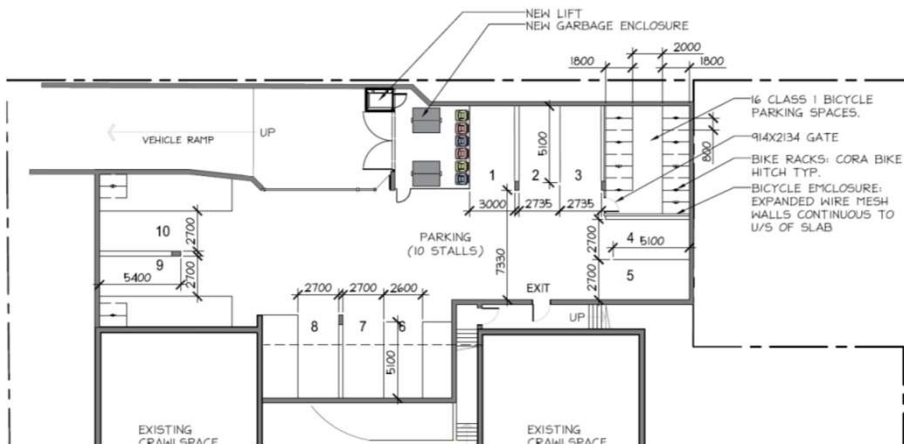
New Underground Parking Configuration Parking Variance: 31 spaces required, 10 proposed
