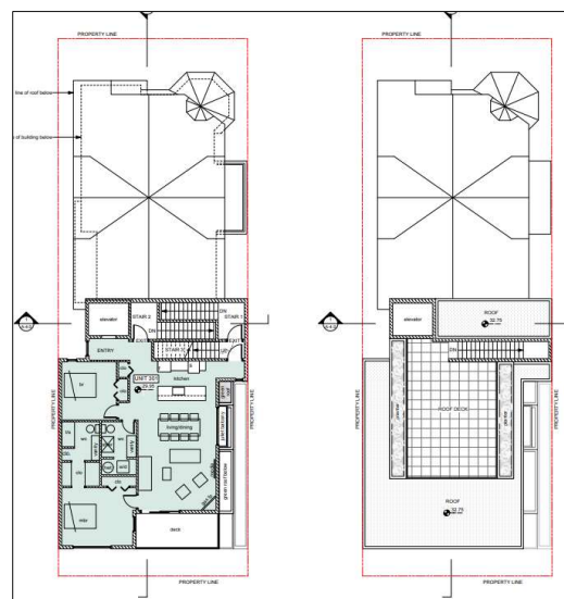
Fourth Storey and Roof Deck
