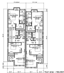
5 Upper Floor Plan - Lot B Scale: 1:100
