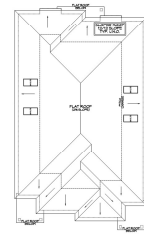
6 Roof Plan - Lot B Scale: 1:100
