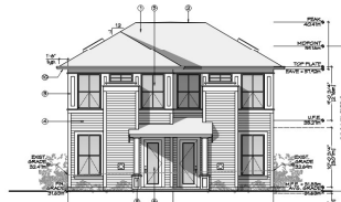
3 Rear Elevation - Lot A Scale: 1:100
