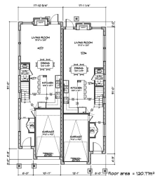
4 Main Floor Plan - Lot B Scale: 1:100
