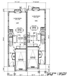
1 Main Floor Plan - Lot A Scale: 1:100
