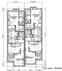
2 Upper Floor Plan - Lot A Scale: 1:100
