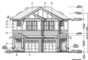
1 Front Elevation - Lot A Scale: 1:100
