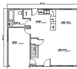
Main Floor Plan
