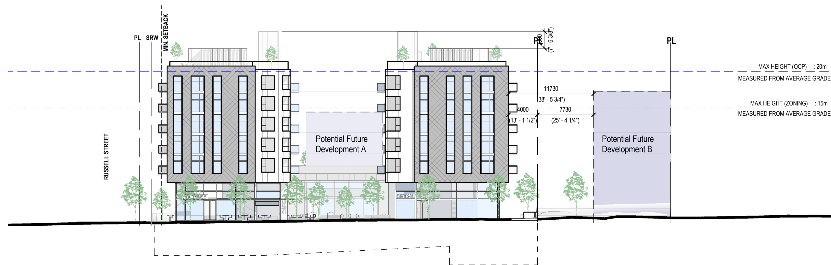
South Elevation
