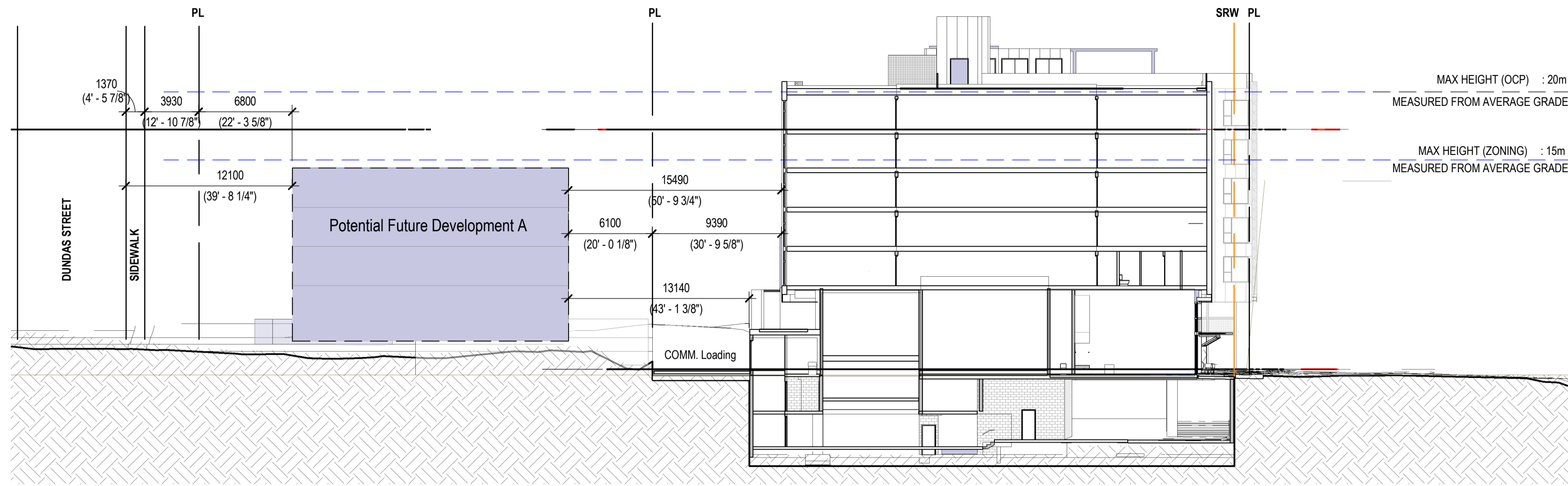
North - South Section Through Residential Tower
