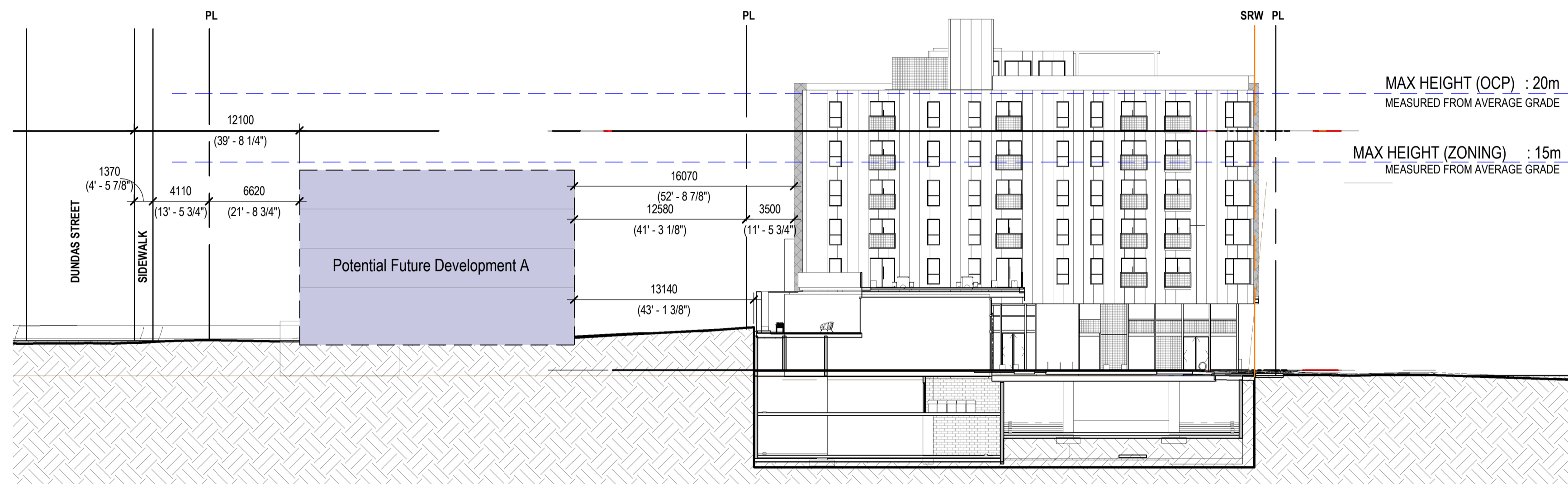
North - South Section Through Commercial Space
