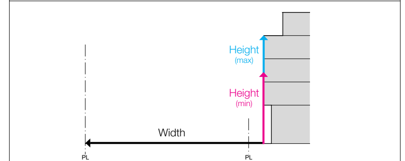
The above example illustrates the minimum and maximum height of the street wall along Quadra Street with a 21.5 m r-o-w + 2 m podium setback. Minimum height = 23.5/2.5 = 9.4 m Maximum height = 23.5/1.6 = 14.7 m
