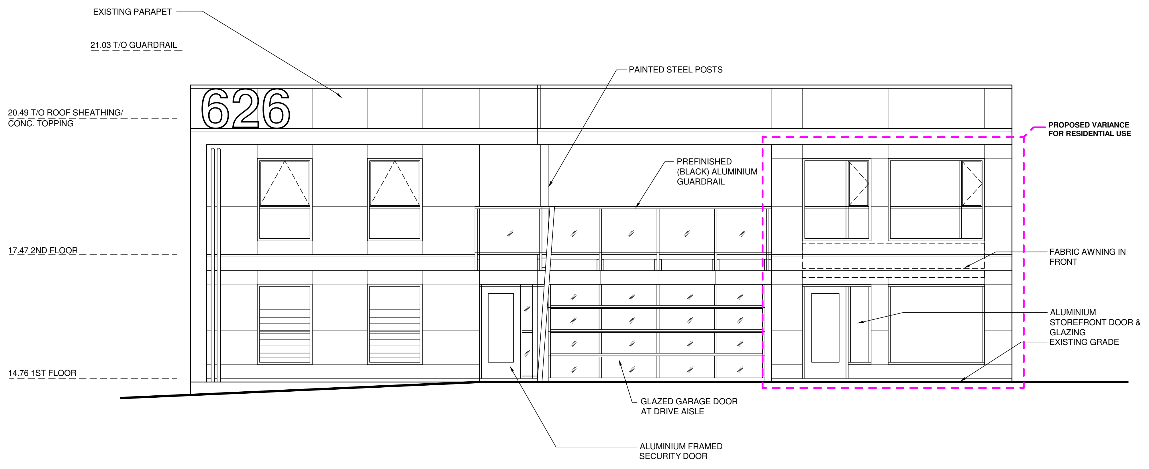
1 Front Elevation (South West) 1/4" = 1'-0"
