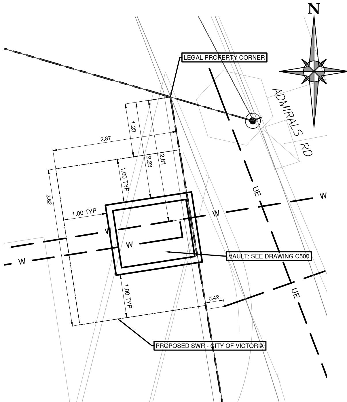
DETAIL A: WATER VAULT ALIGNMENT AND EASEMENT
