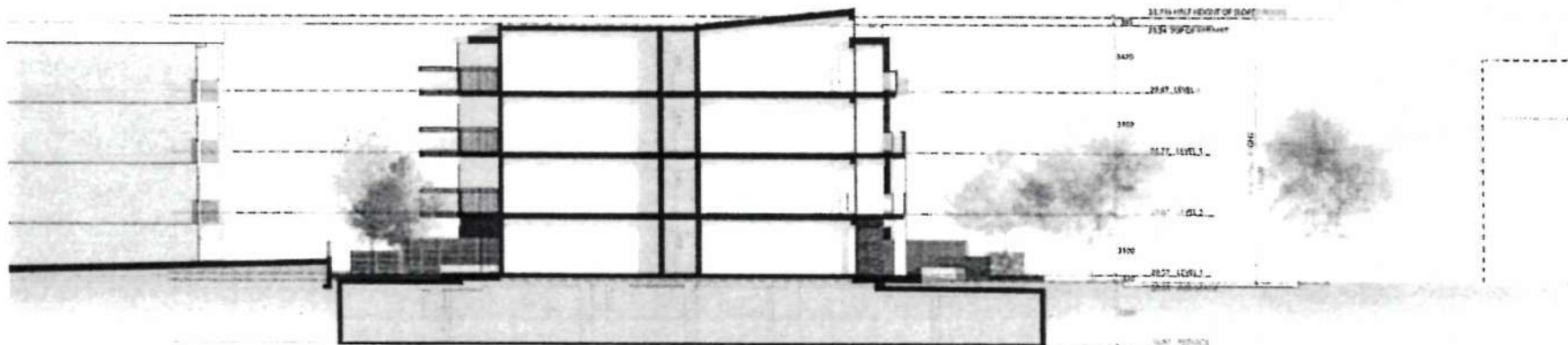
B B WEST FACING NORTH-SOUTH BLD'G SECTION 1:100
