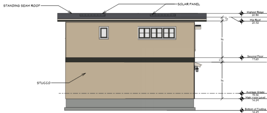
② NORTH SIDE ELEVATION SCALE 1/8"=1' 0"
