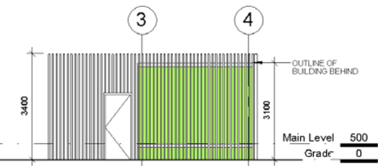
North Elevation
