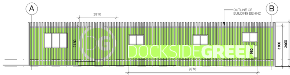
West Elevation
