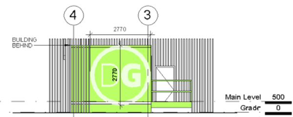
South Elevation
