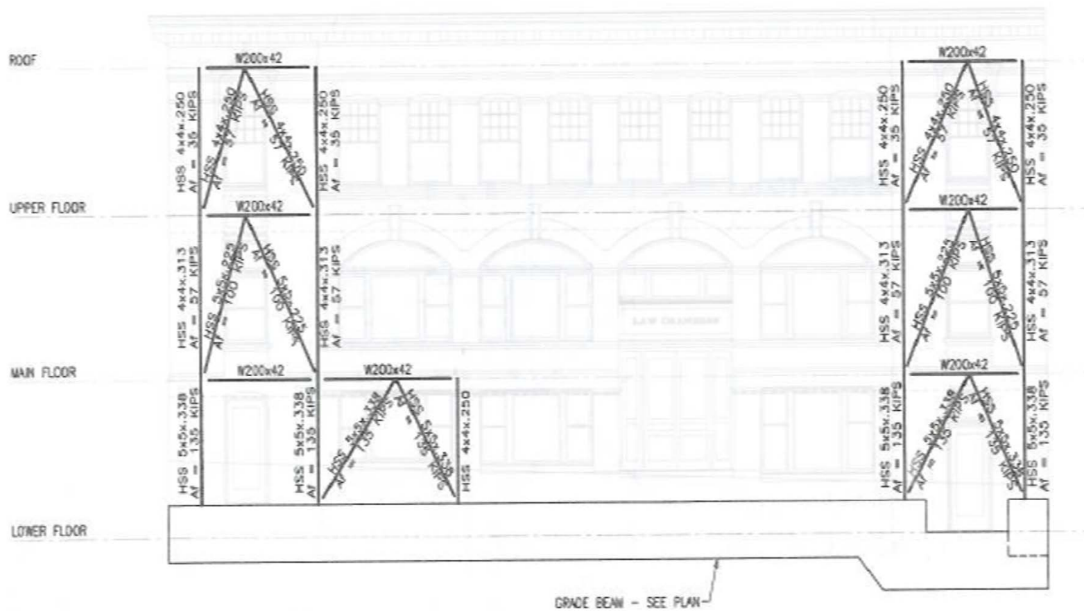
1 NORTH ELEVATION SSK-03
