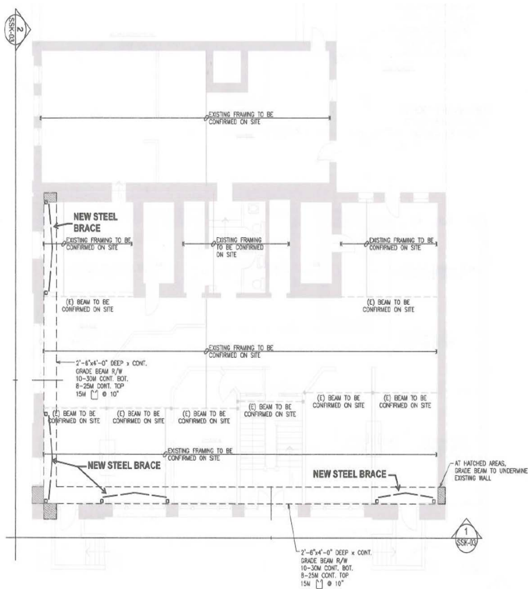
Lower Floor Plan
