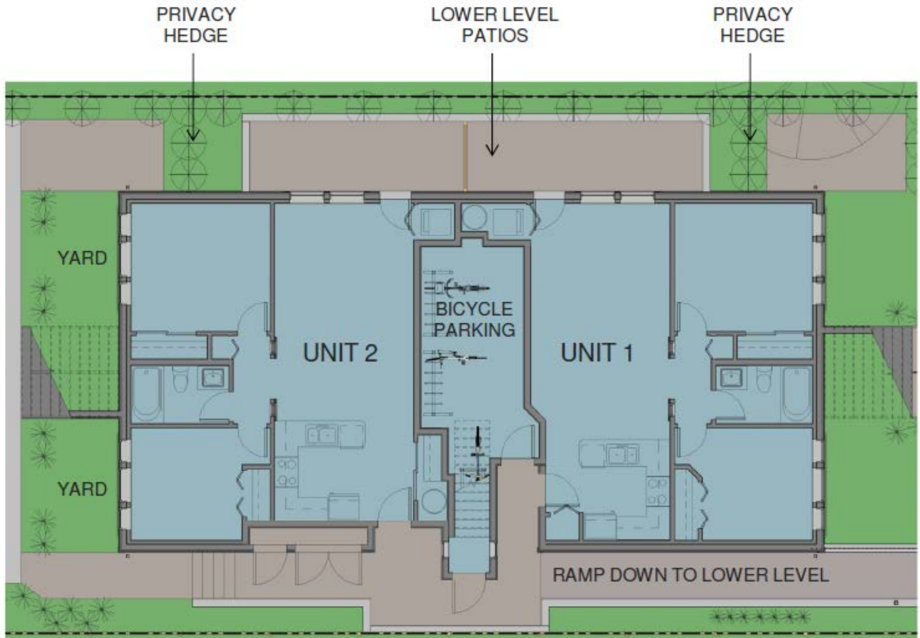
Lower Level
