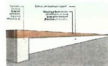
WOOD TOP W/ GALVANIZED METAL & CONCRETE CUSTOM BENCH DESIGN
