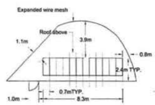
BIKE ENCLOSURE DETAIL scale 1/8" = 1'-0"
