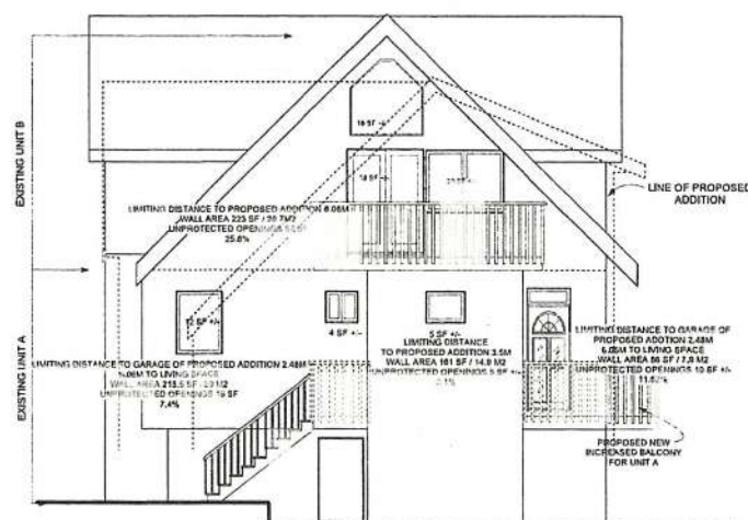
SOUTH ELEVATION
