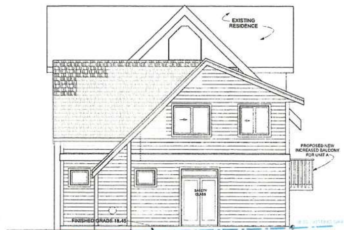
LEFT ELEVATION PROPOSED SCALE: 1/4"=1'-0"
